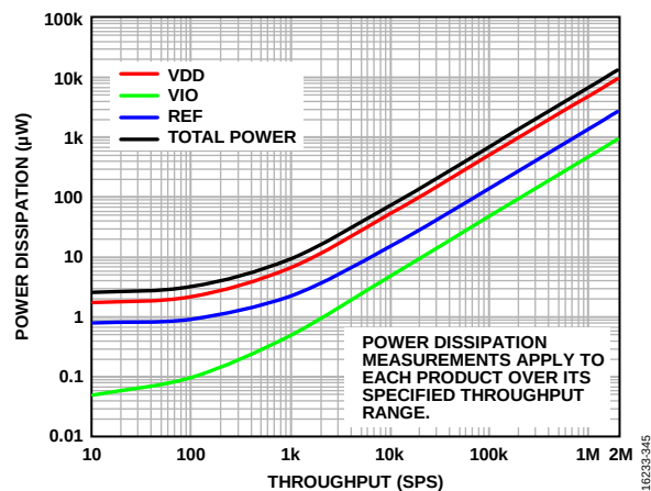
Figure 46. Power Dissipation vs. Throughput, V_{\text{DD}} = 1.8 \text{ V} , V_{\text{IO}} = 1.8 \text{ V} , V_{\text{REF}} = 5 \text{ V} , T_A = 25^\circ\text{C}
