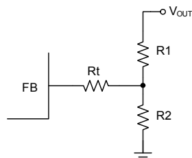
Figure 2—Feedback Network
