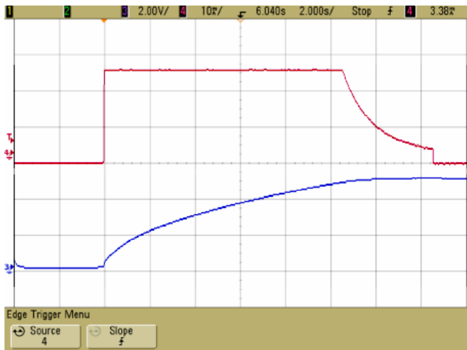
Figure 3. Charging Mode, V_{SYS} 2.5V, Input Current Set to 0.5A, Ch 4 (Red) Input Current, 200mA/DIV, Ch3 (Blue) VCAP Voltage
