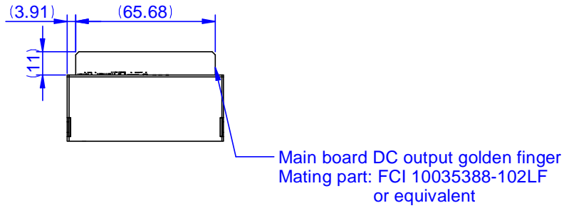
Figure 17 - Mating Connector
