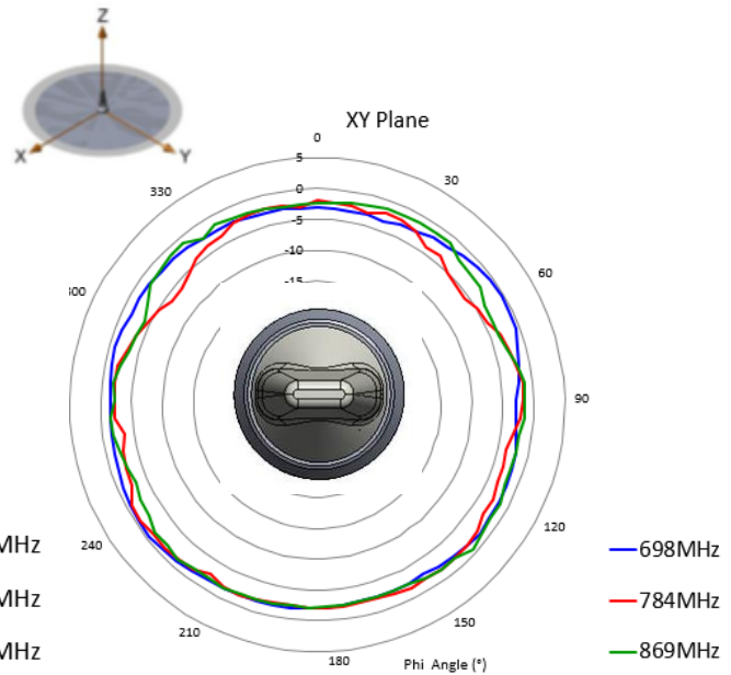
Horizontal Plane
