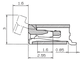
SECT X-X
