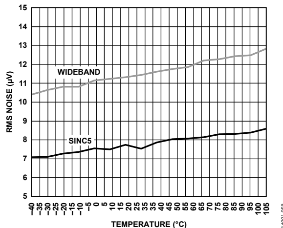
Figure 29. RMS Noise vs. Temperature, Fast Mode
