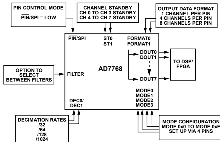
Figure 76. AD7768 Pin Configurable Functions
