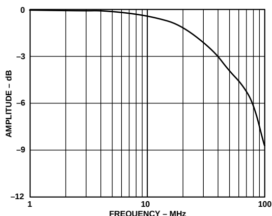
Figure 22. Full-Power Bandwidth
