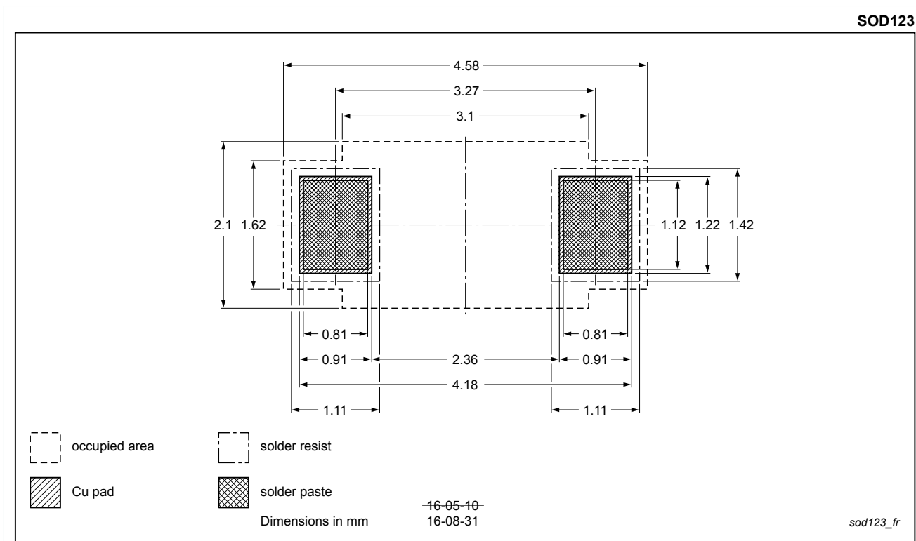
Figure 9. Reflow soldering footprint SOD123
