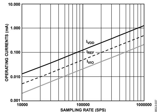
Figure 28. Operating Currents vs. Sampling Rate
