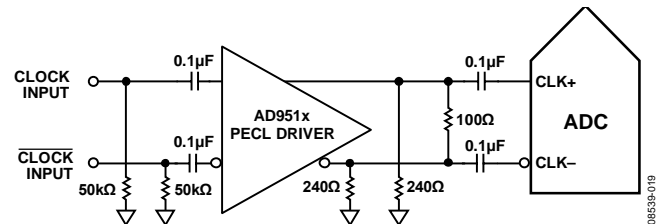
Figure 49. Differential PECL Sample Clock (Up to 4× Rated Sample Rate)
