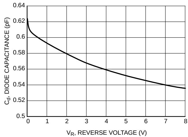
Figure 4. Diode Capacitance
