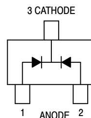
SC-59 CASE 318D STYLE 3
