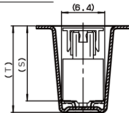
SECT. F-F
