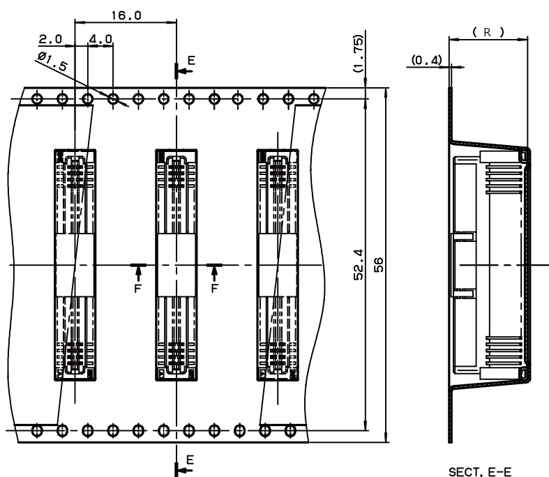
SECT. E-E
