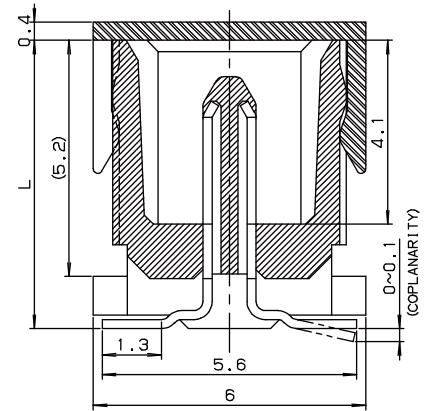
SECT. A-A
