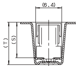
SECT. F-F
