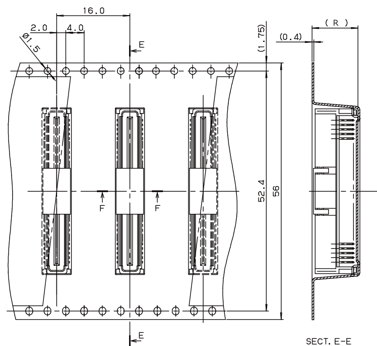
SECT. E-E
