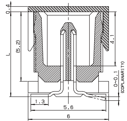
SECT. A-A
