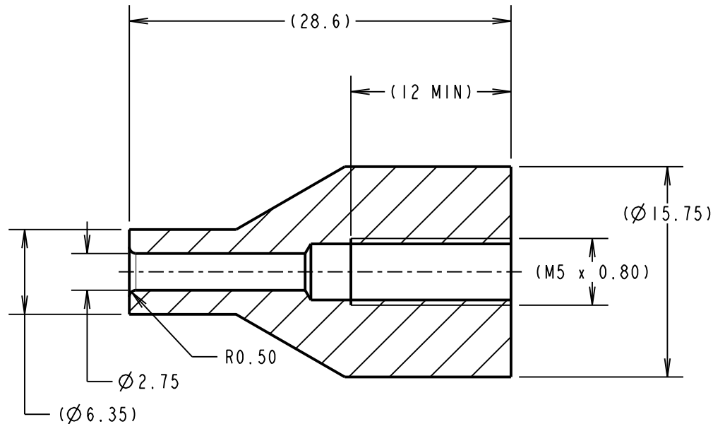
Z10000-00 BOTTOM TOOL PART MACHINED BLANK
