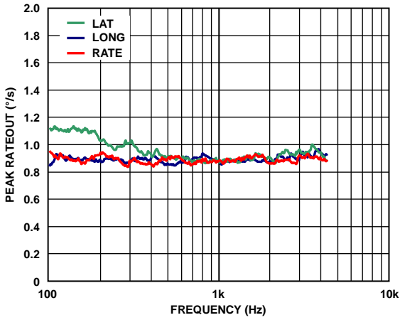
Figure 16. Typical Response to 10 g Sinusoidal Vibration (Sensor Bandwidth = 40 Hz)
