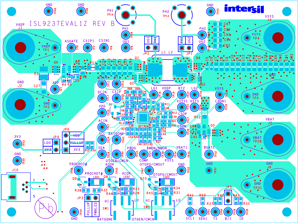
FIGURE 9. TOP LAYER
