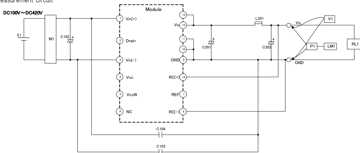
Measurement circuit
