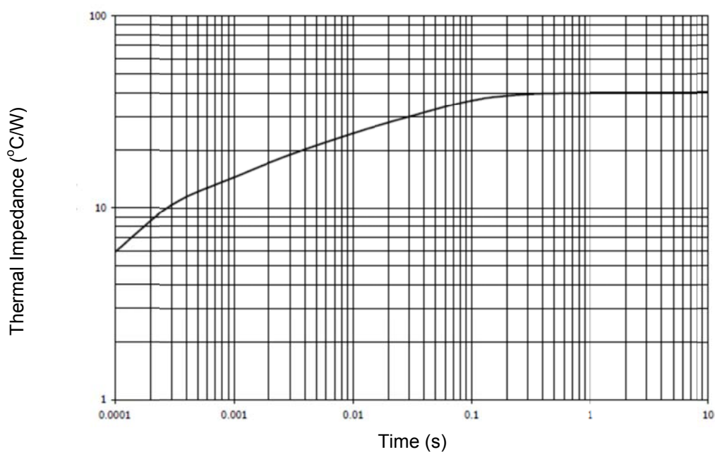
FIGURE 3 Maximum Thermal Impedance at T_{EC} = 25^{\circ}\text{C}
