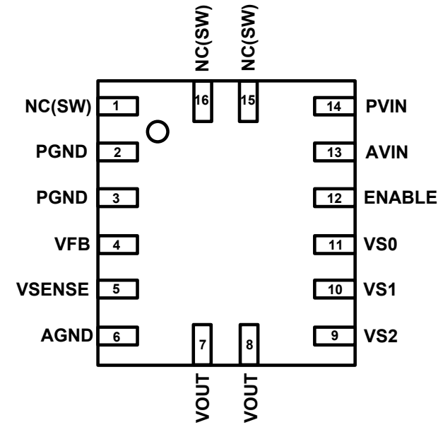
Figure 3: EP5358LUA Pin Out Diagram (Top View)
