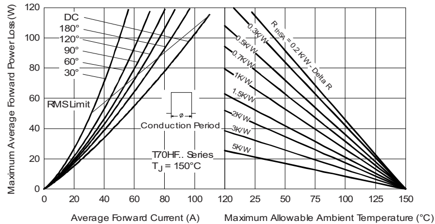
Fig. 10 - Forward Power Loss Characteristics
