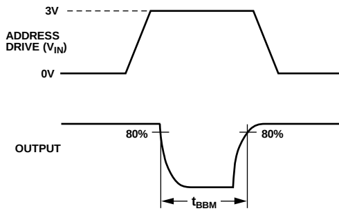
Figure 37. Break-Before-Make Time Delay, t_{BB}
