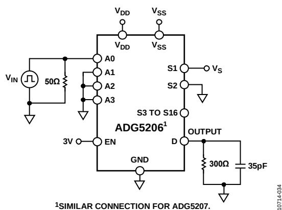
Figure 35. Address to Output Switching Times, t_{TRANSITION}
