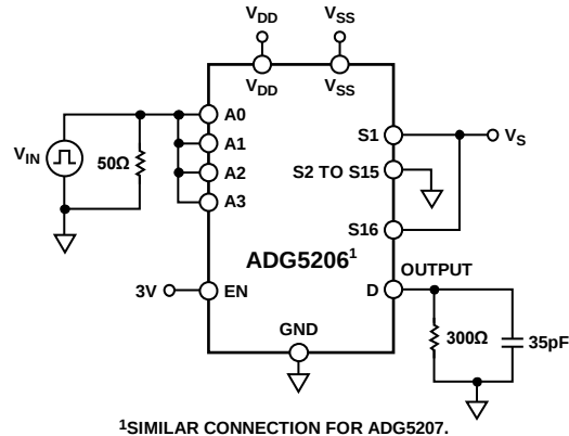
Figure 37. Break-Before-Make Time Delay, t_{BB}
