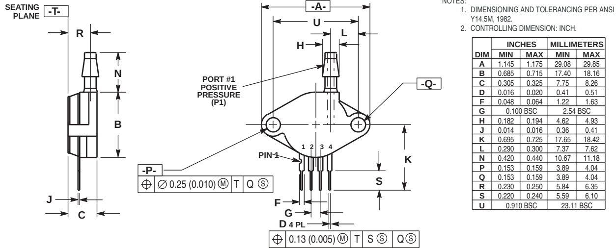
Case 98ASB14911C, Unibody package
