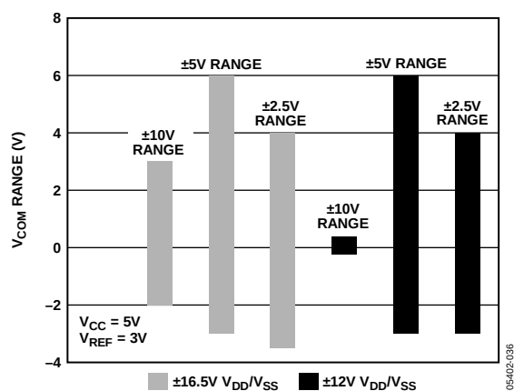
Figure 39. Common-Mode Range for V_{CC} = 5V and REF_{IN}/REF_{OUT} = 3V
