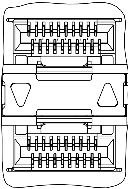
OUTER LIGHT PIPES 2198325-4, 2198325-8 SCALE 5:1
