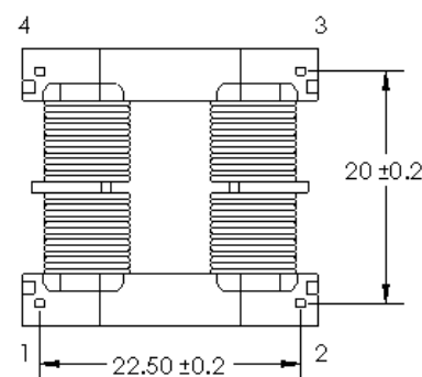
BOTTOM DRAWING
