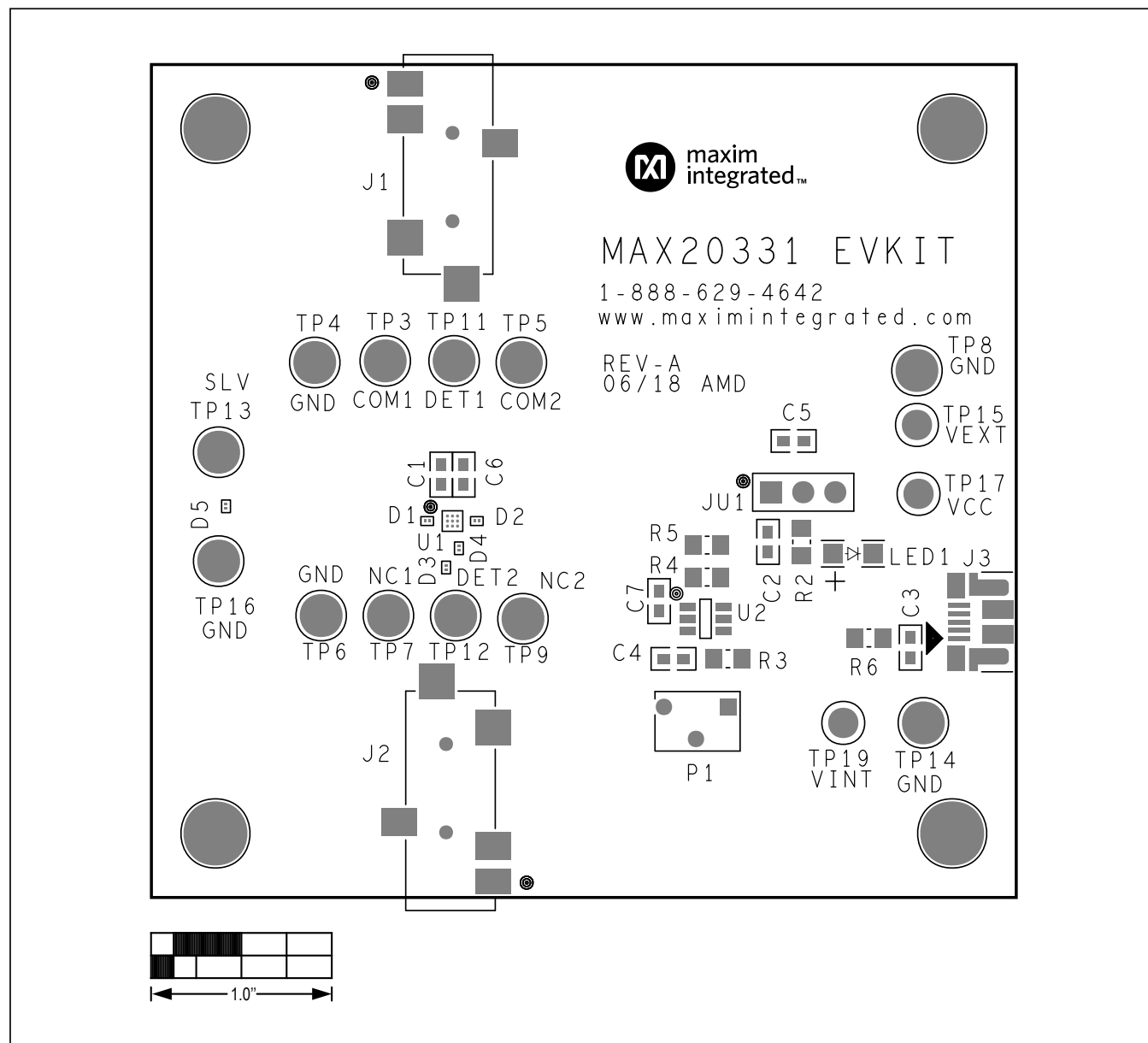
MAX20331 EV Kit—Top Silkscreen
