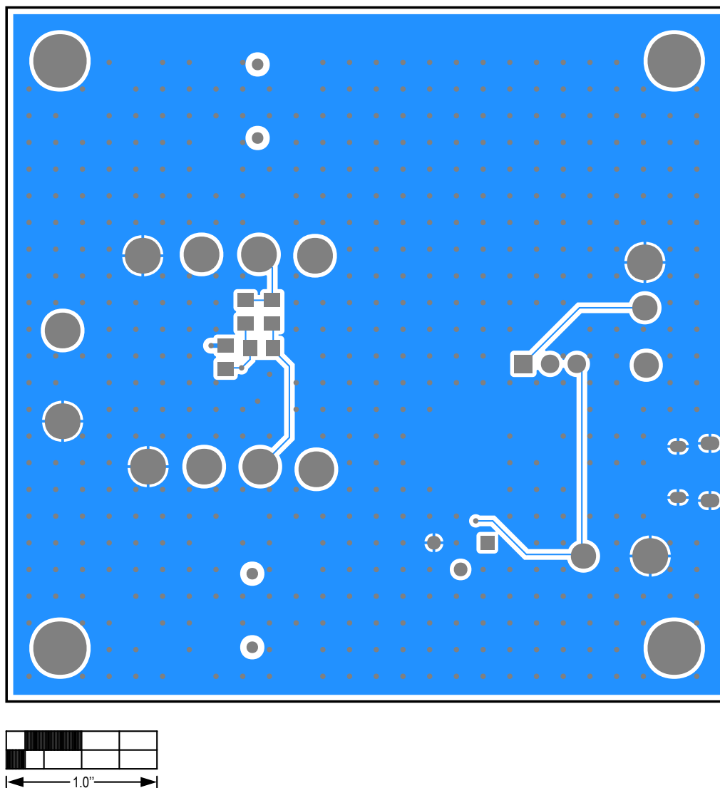
MAX20331 EV Kit—Bottom
