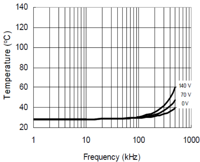
Figure 33. IRS21864S vs. Frequency (IRFBC20) R_{\text{gate}} = 33\Omega , V_{\text{CC}} = 15\text{V}
