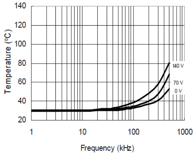
Figure 34. IRS21864S vs. Frequency (IRFBC30) R_{\text{gate}} = 22\Omega , V_{\text{CC}} = 15\text{V}
