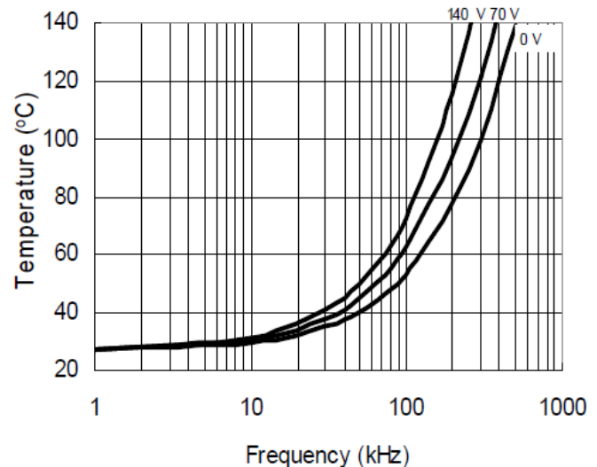
Figure 36. IRS21864S vs. Frequency (IRFPE50) R_{\text{gate}} = 10\Omega , V_{\text{CC}} = 15\text{V}
