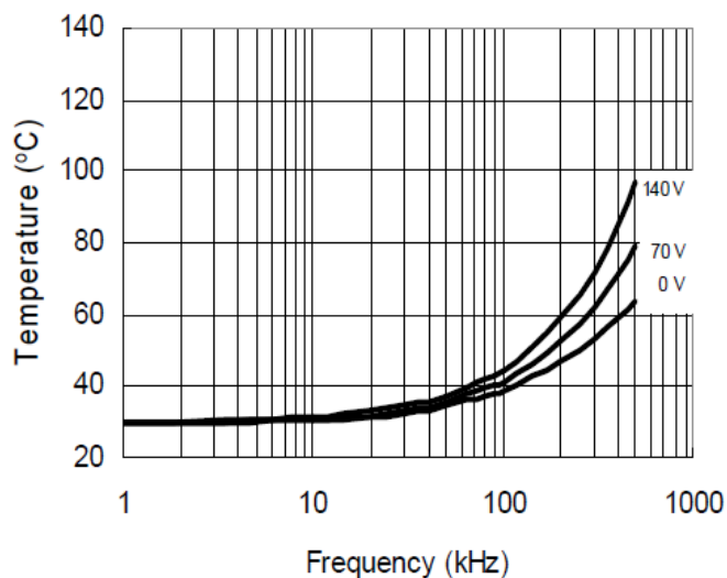
Figure 35. IRS21864S vs. Frequency (IRFBC40) R_{\text{gate}} = 15\Omega , V_{\text{CC}} = 15\text{V}
