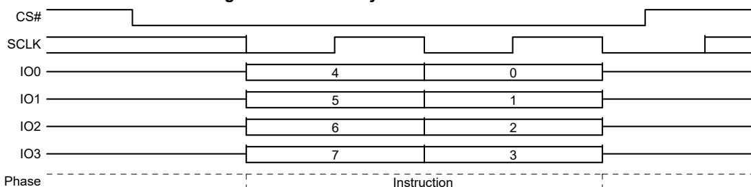
Figure 71. Enter 4 Byte Address QPI Mode
