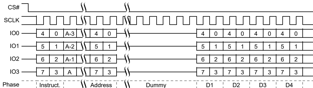
Figure 50. RSFDP QPI Mode Command Sequence
