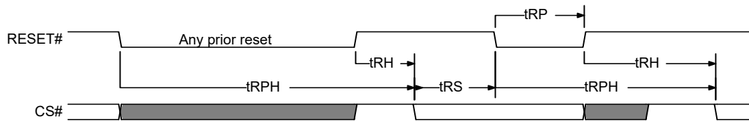
Figure 28. Hardware Reset using RESET# Input
