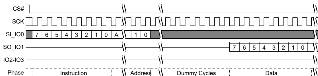
Figure 72. Read Any Register Read Command Sequence
