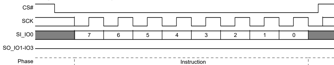
Figure 70. Enter 4 Byte Address Mode (4BEN B7h) Command Sequence
