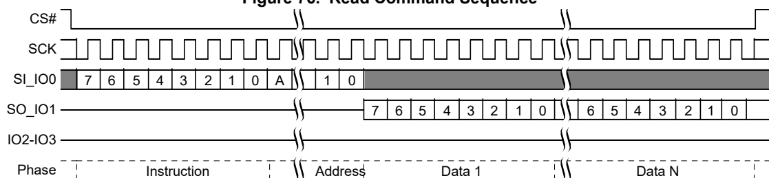
Figure 76. Read Command Sequence
