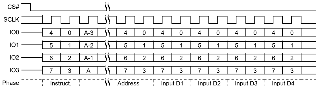
Figure 109. DYB Write QPI Mode Command Sequence
