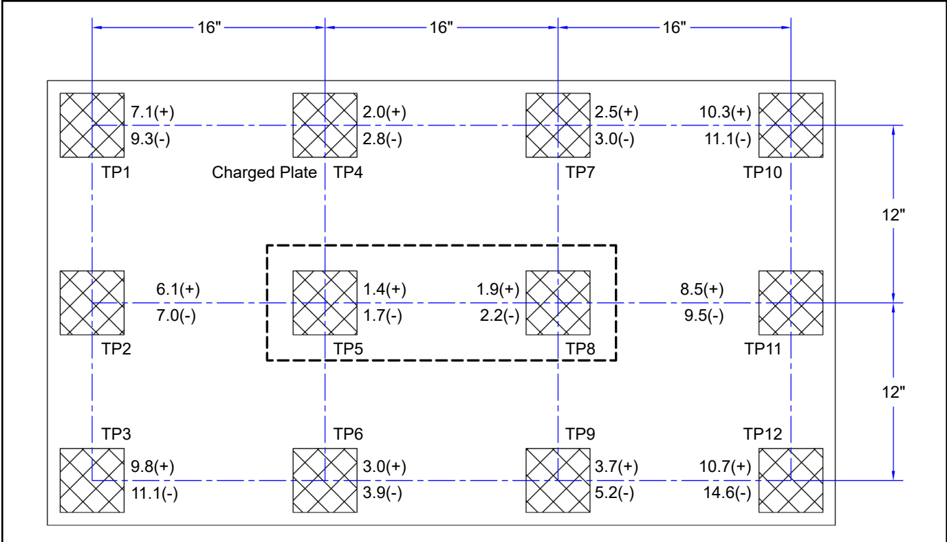
Figure 10. 770112 Neutralization (Discharge) Times at 120VAC, 60Hz input
