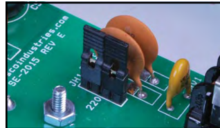
Figure 5. 120 VAC jumper setting
