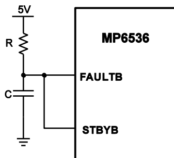
FIGURE 2. Fault Protection Enhancement Circuit
