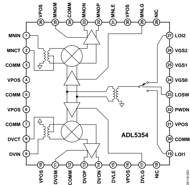
Figure 51. Simplified Schematic
