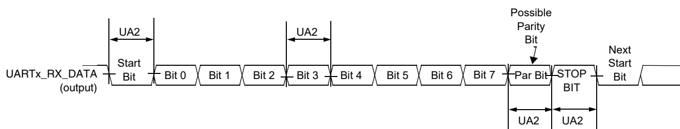
Figure 46. UART RS-232 Serial mode receive timing diagram
