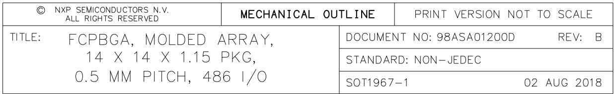
Figure 47. 14 X 14 MM BGA, case x package top, bottom, and side views
