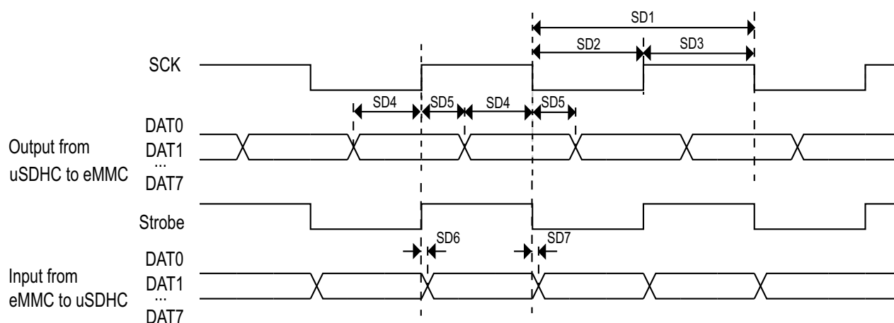
Figure 14. HS400 timing
