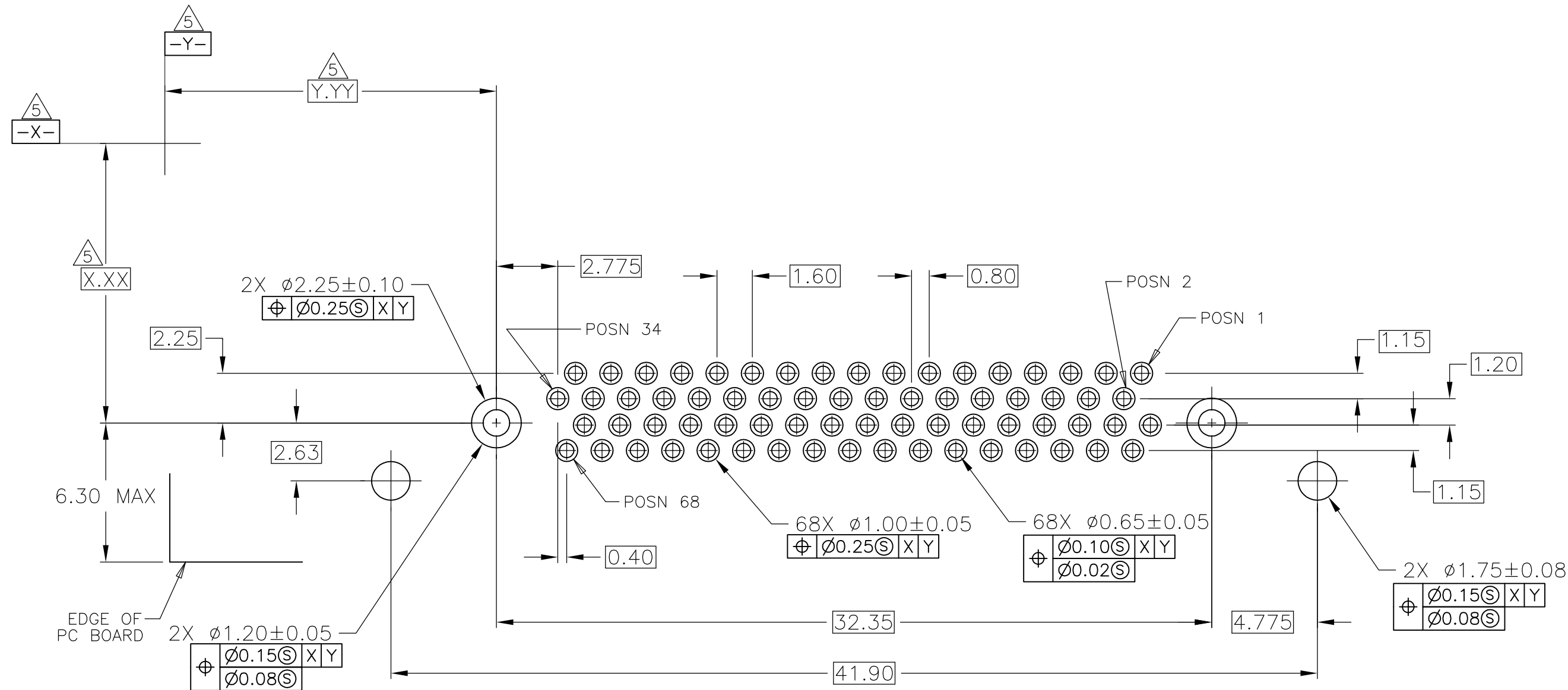
PC BOARD MOUNTING DIMENSIONS
