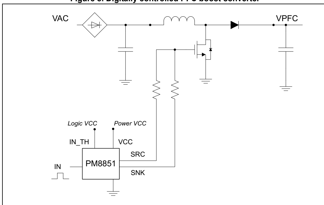
Figure 8. Digitally controlled PFC boost converter
