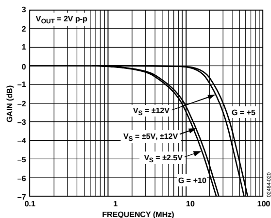
Figure 19. AD8130 Frequency Response vs. Supply, G = +5 , G = +10 , V_{OUT} = 2\text{ V p-p}
