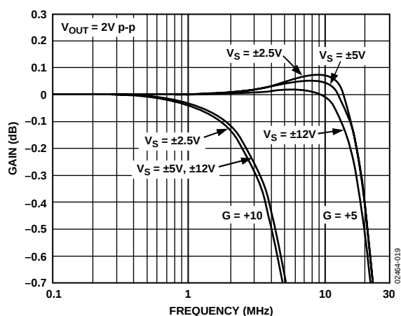
Figure 18. AD8130 Fine Scale Response vs. Supply, G = +5 , G = +10 , V_{OUT} = 2\text{ V p-p}
