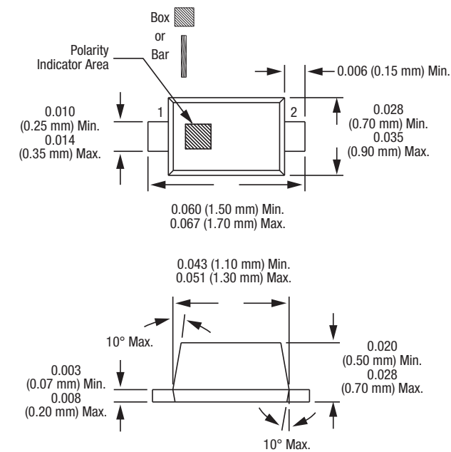
Figure 5. SC-79 Package Dimension Drawing
