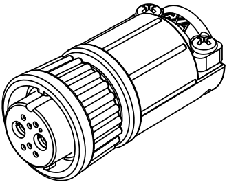
STD COUPLING RING P/N: W3B80-8SG-5XX
