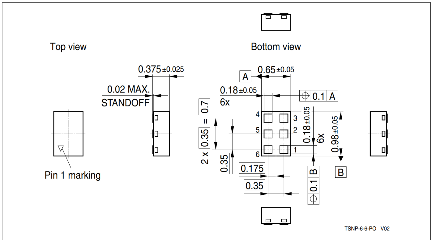
Figure 3: Package Outline
