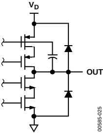
Figure 25. Equivalent Reference Output Circuit
