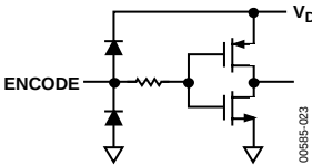
Figure 23. Equivalent Encode Input Circuit
