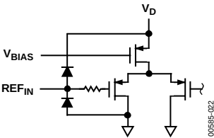
Figure 22. Equivalent Reference Input Circuit
