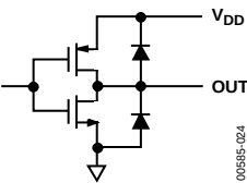
Figure 24. Equivalent Digital Output Circuit
