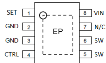
MSOP-8EP
