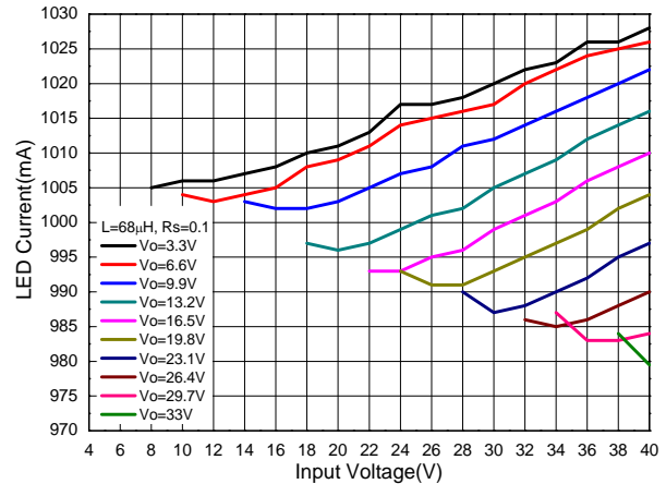
LED Current vs. Input Voltage (MSOP-8EP, Rs=0.1Ω, L=68μH)
