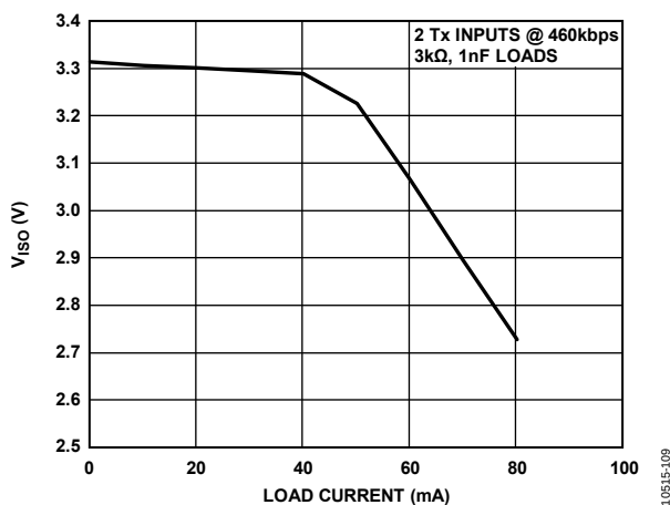
Figure 11. V_{ISO} vs. V_{ISO} Load Current
