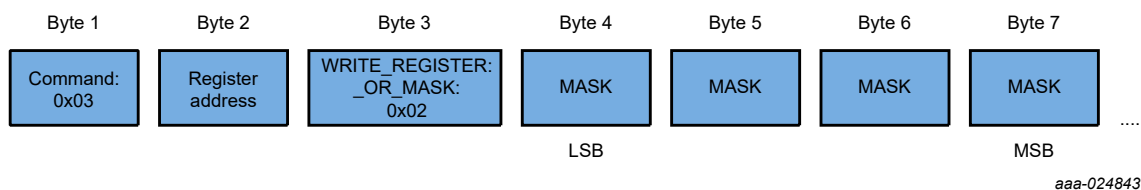
Figure 14. WRITE_REGISTER_OR_MASK
