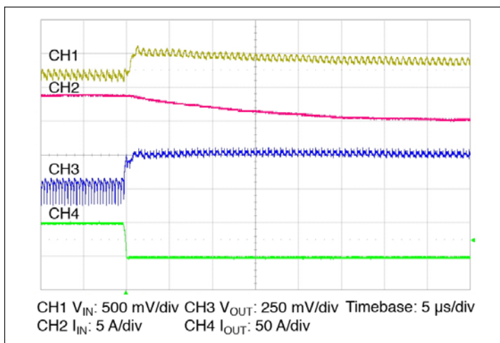
Figure 12 — 50 A – 0 A transient response: C_{IN} = 330 \mu F , I_{IN} measured prior to C_{IN} , no external C_{OUT}
