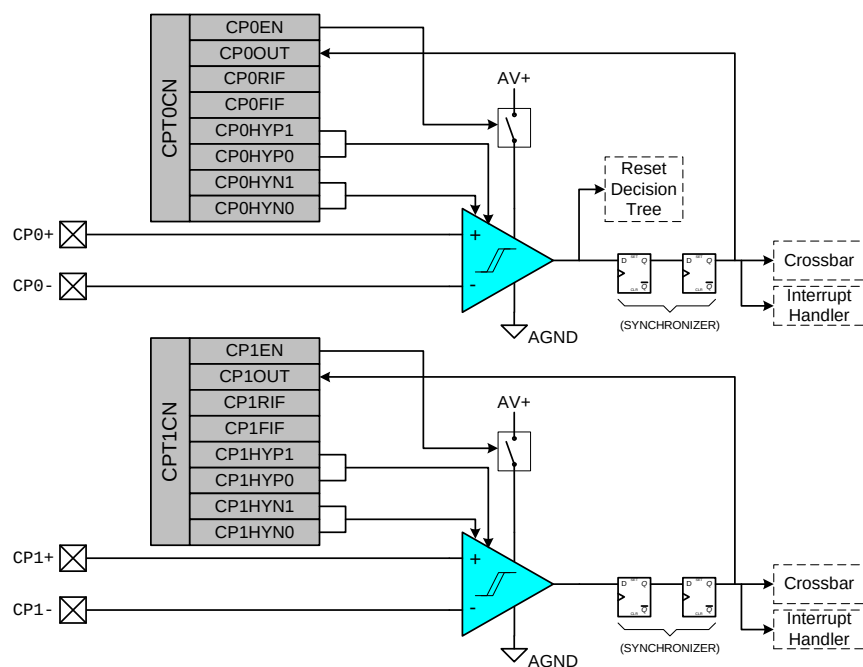
Figure 11.1. Comparator Functional Block Diagram
